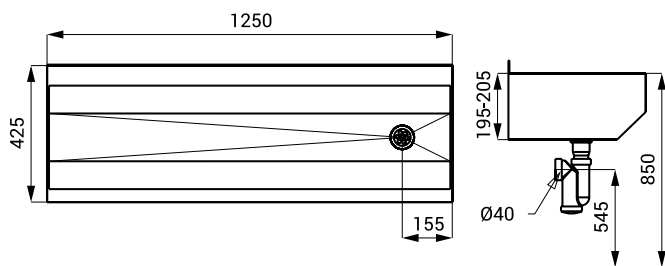
SLUN 10, 10L
