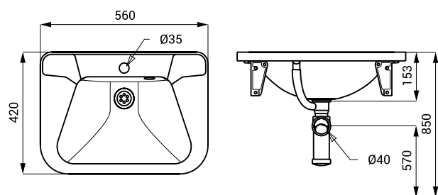
SLUN 26, 26A
