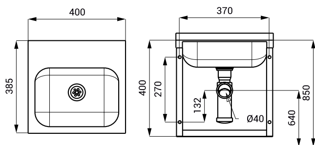
SLUN 13
