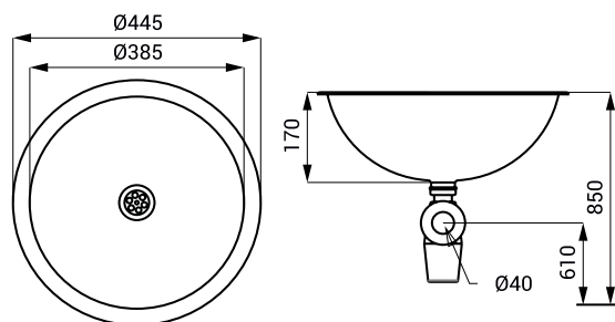
SLUN 34
