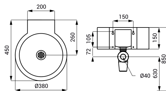
SLUN 17
