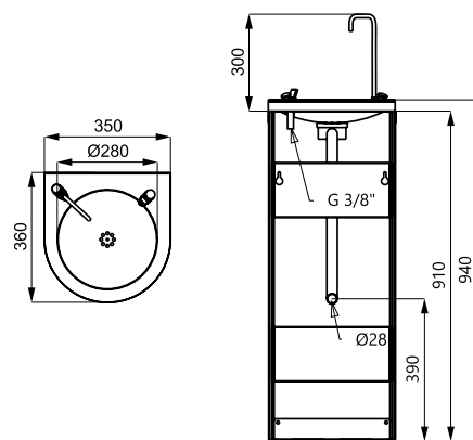
SLUN 43S
