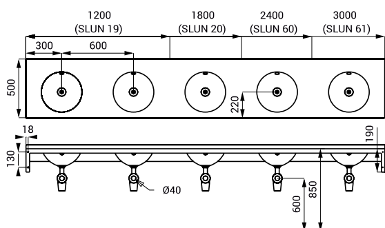
SLUN 19, 20, 60, 61
