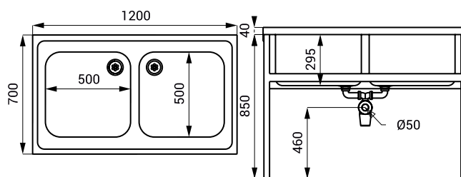
SLUN 16
