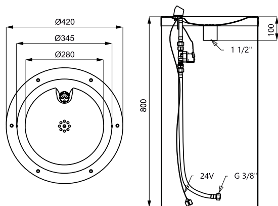
SLUN 23, 23E
