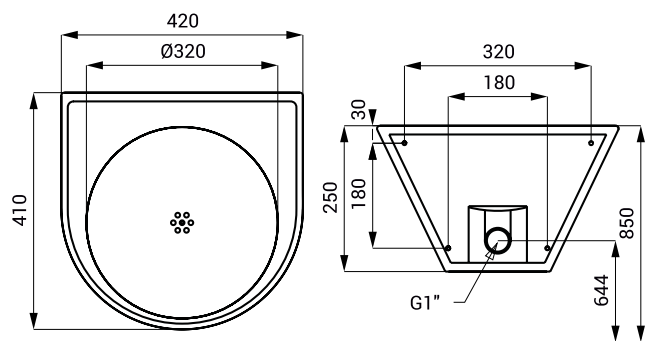
SLUN 22M
