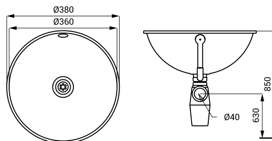
SLUN 45, 45X
